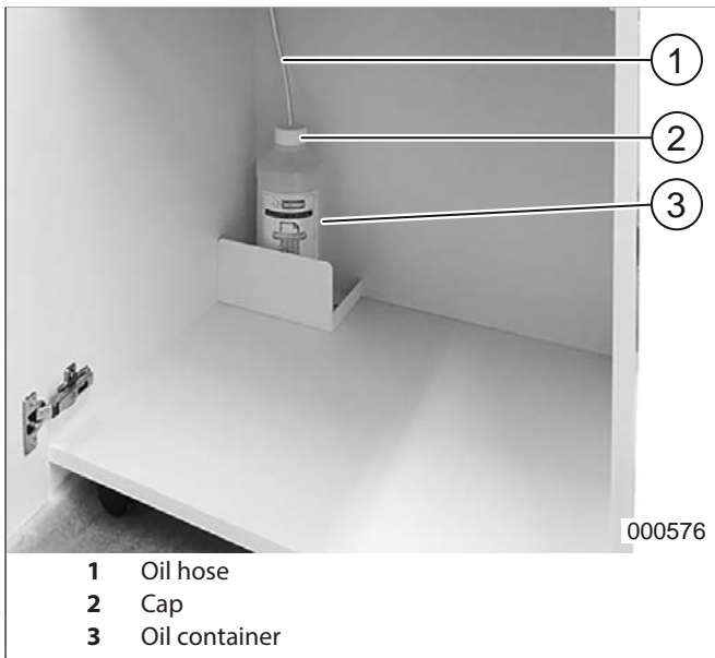
fig.6 Oil container
