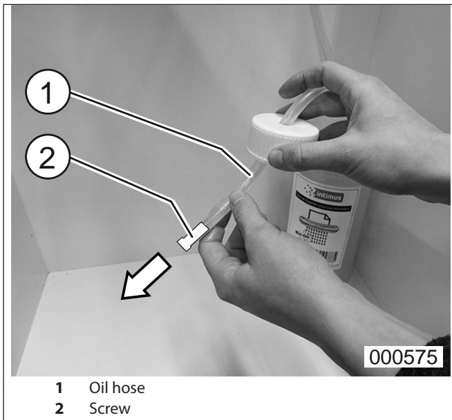
fig. 1 Oiler installation
